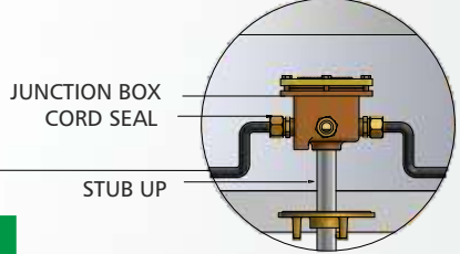
Underwater Junction box Installation Detail For Base or Yoke Mount Fixtures
